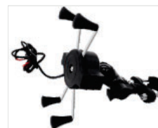
Model: YL-EC20 Material: PC+Stainless steel+Aluminum alloy Input: 30-150V Output: 5V 2.4A Fit for: Electric bike/motorcycle/tricycle Installation: Electric Bike Handlebar Qty/Ctn: 50PCS
