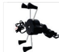
Model: YL-EC20 Material: PC+Stainless steel+Aluminum alloy Input: 30-150V Output: 5V 2.4A Fit for: Electric bike/motorcycle/tricycle Installation: Electric Bike Rear Mirror Qty/Ctn: 50PCS
