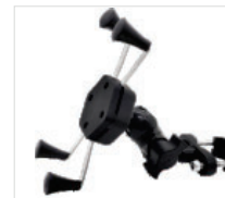
Model: YL-MH05-CZ Material: Nylon+Stainless steel+Aluminum alloy Fit for: Motorcycle/Electric Bike/Bike Installation: Motorcycle/Electric Bike /Bike Handlebar Qty/Ctn: 50PCS
